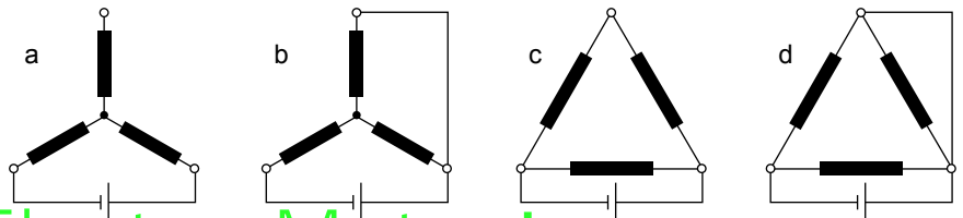
Electro_Motor.ir Motor winding connections for D.C. voltage
